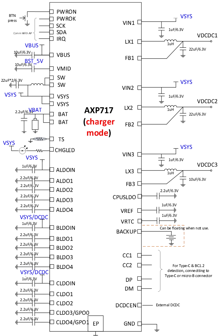
Figure 7-1 Charger Mode Application
