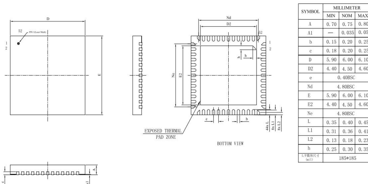
Figure 8-2 AXP717 Marking
