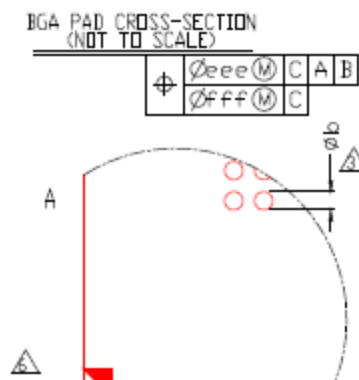
Figure 3- Package Outline Drawing – bottom view
