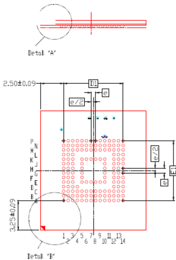
Figure 2 - INAND 7232 Specification Top and Side View (Detail A)
